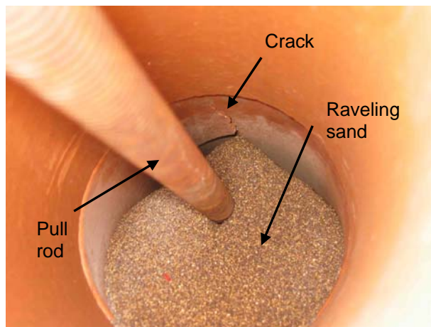
Figure 5. Photograph showing an internal view of the clay pipe with a crack near the pipe crown.
